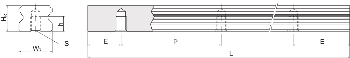
(5) Dimensions for ER-T (rail mounting from bottom)
