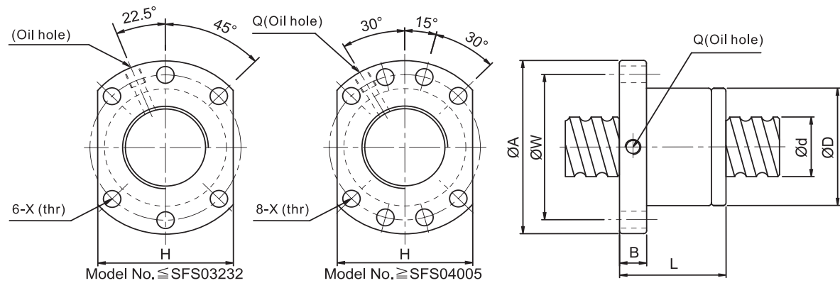
2-2 Size Table of SFS Ball Screws
