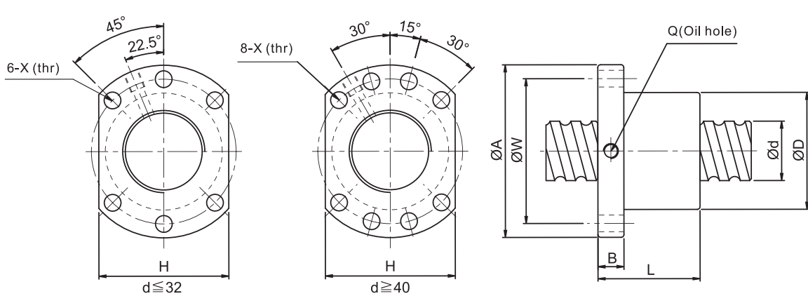
2-3 Size Table of SFNU Ball Screws
